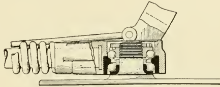
Fig. 103. Ball-Bearing of Fig. 102 in Detail
